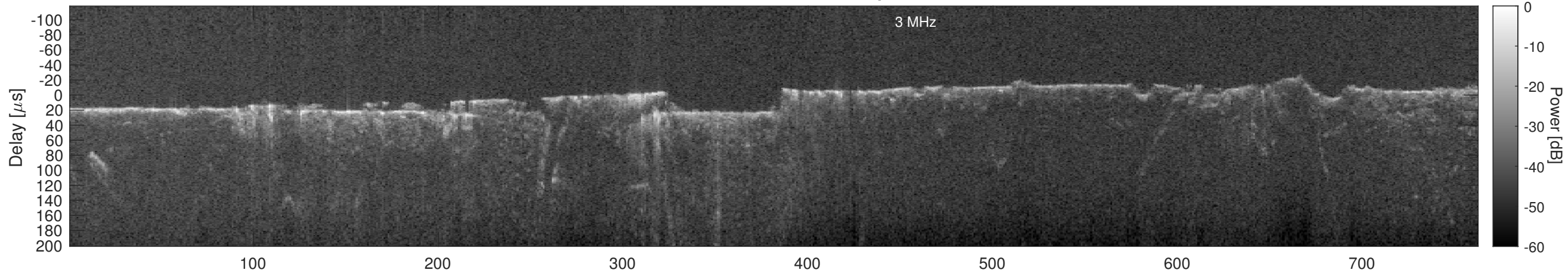
Orbit 4953, Cluttergram
