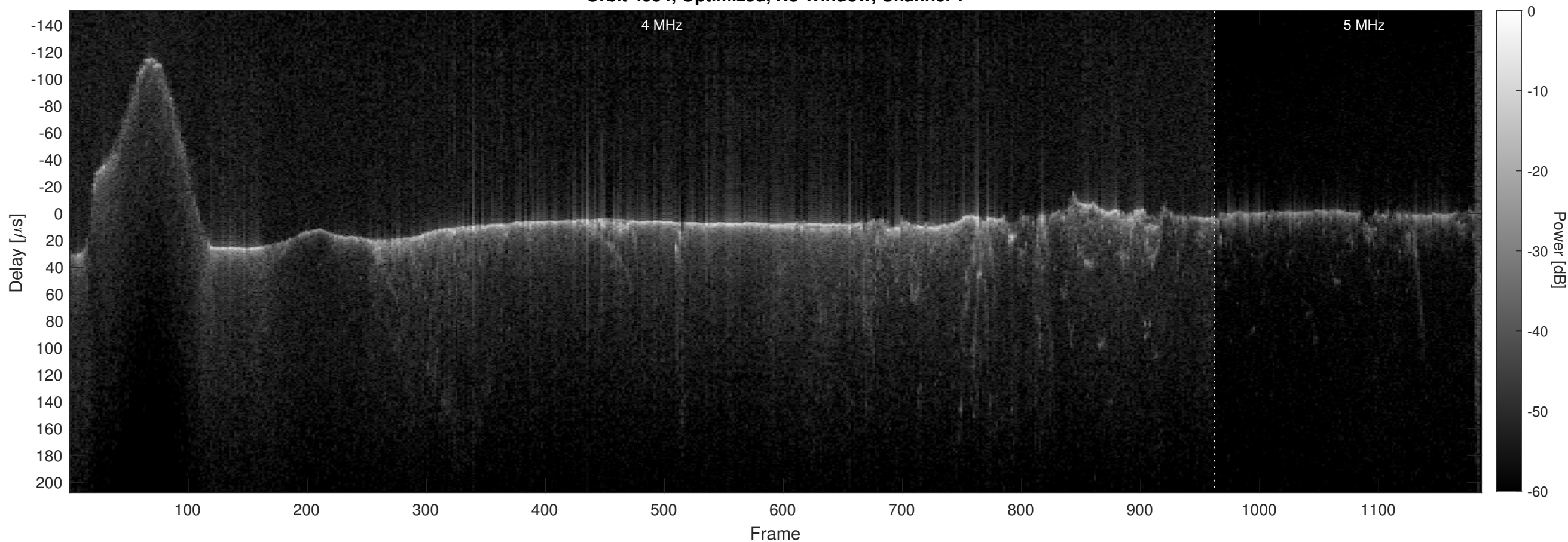
Orbit 4954, Optimized, No Window, Channel 2
