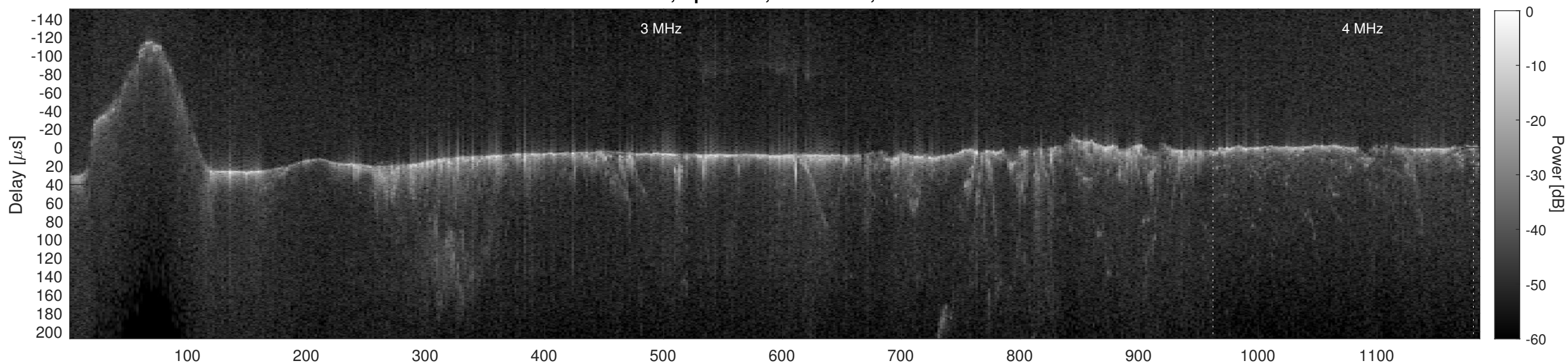
Orbit 4954, Cluttergram
