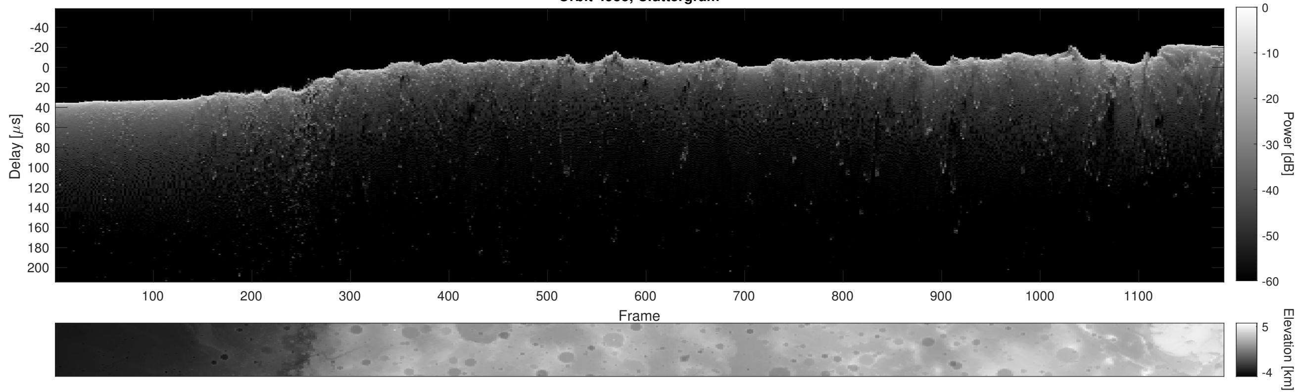
Orbit 4955, Cluttergram
