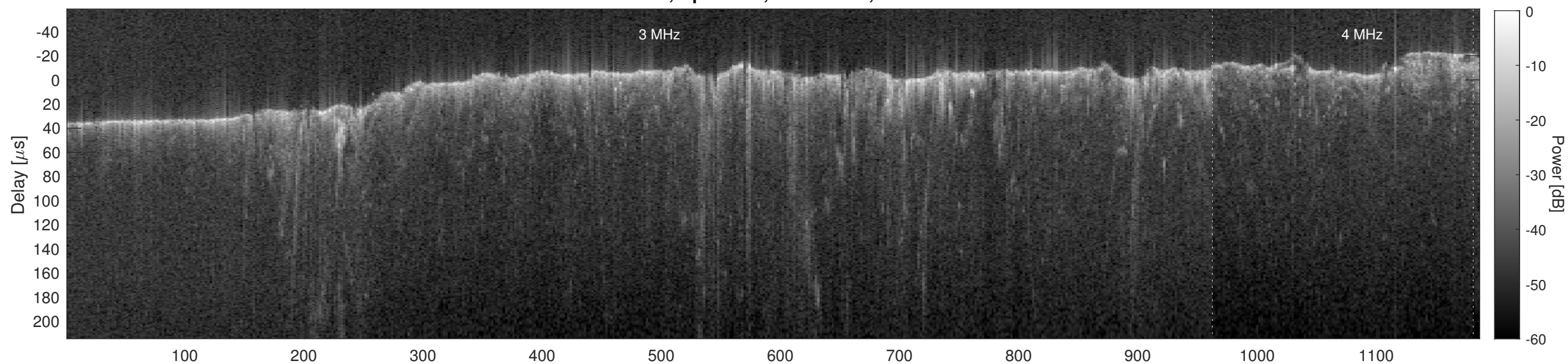
Orbit 4955, Cluttergram
