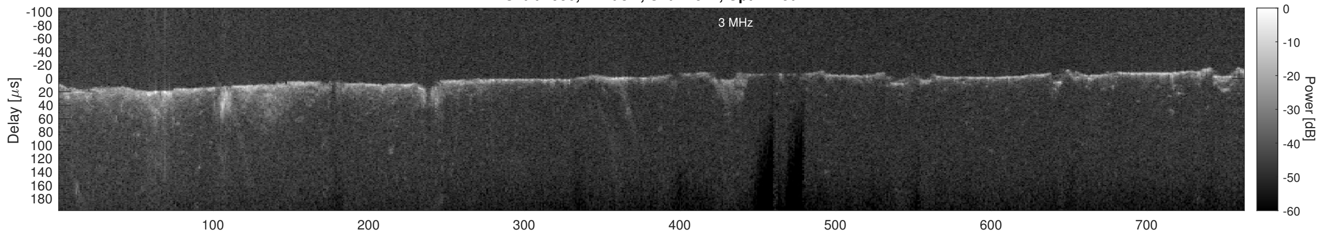
Orbit 4956, Cluttergram
