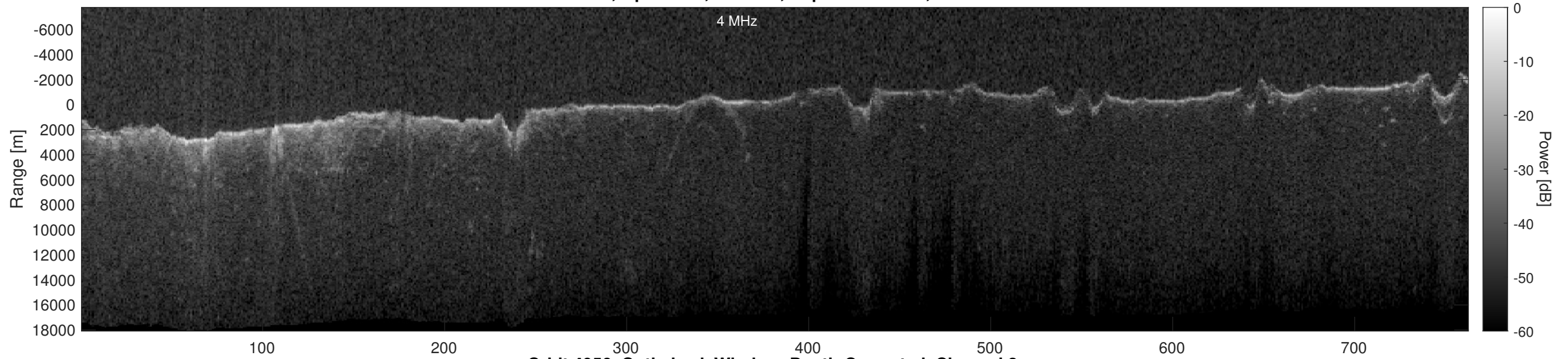
Orbit 4956, Optimized, Window, Depth-Corrected, Channel 2
