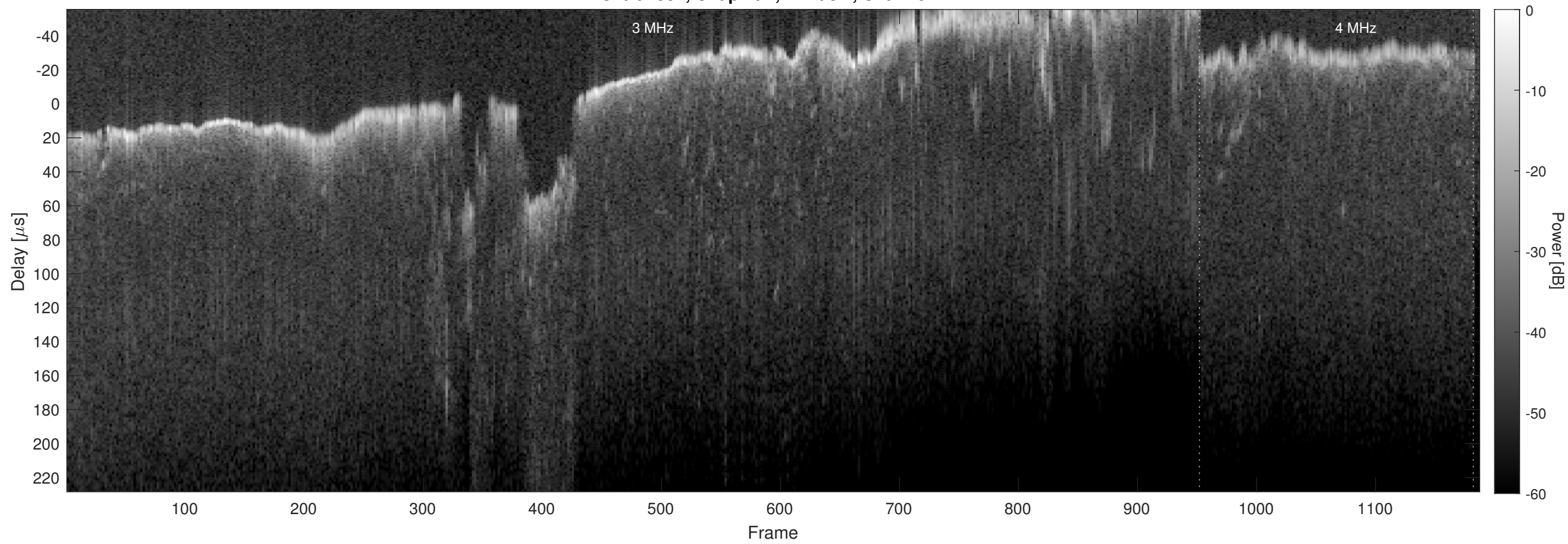
Orbit 4957, Chapman, Window, Channel 2
