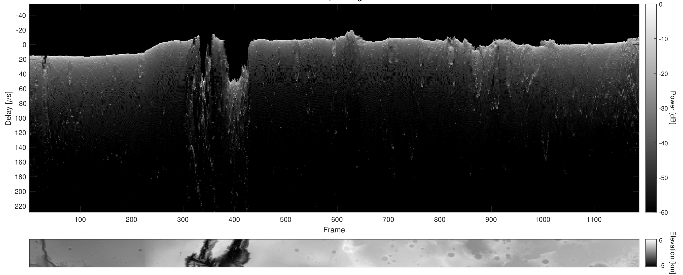
Orbit 4957, Cluttergram
