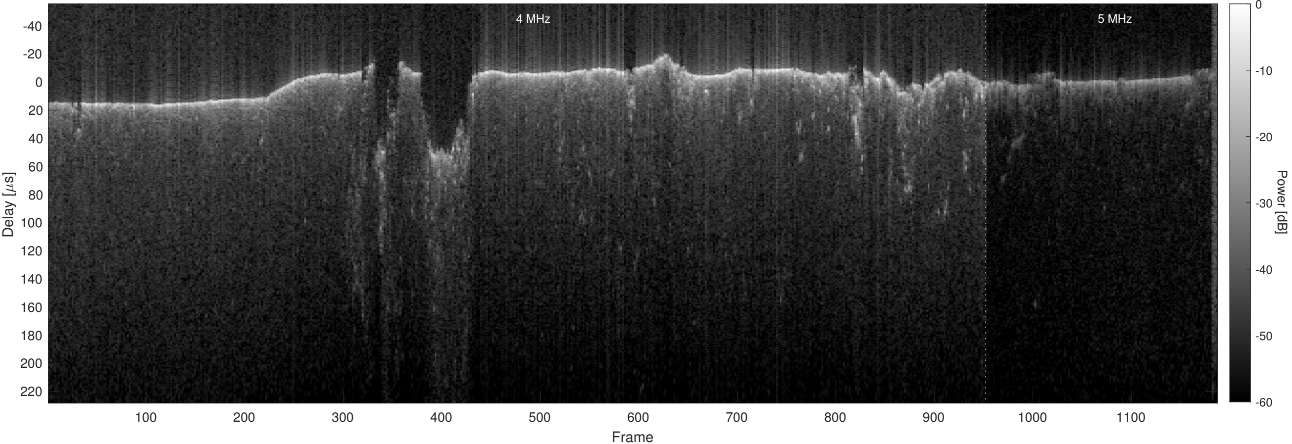
Orbit 4957, Optimized, No Window, Channel 2
