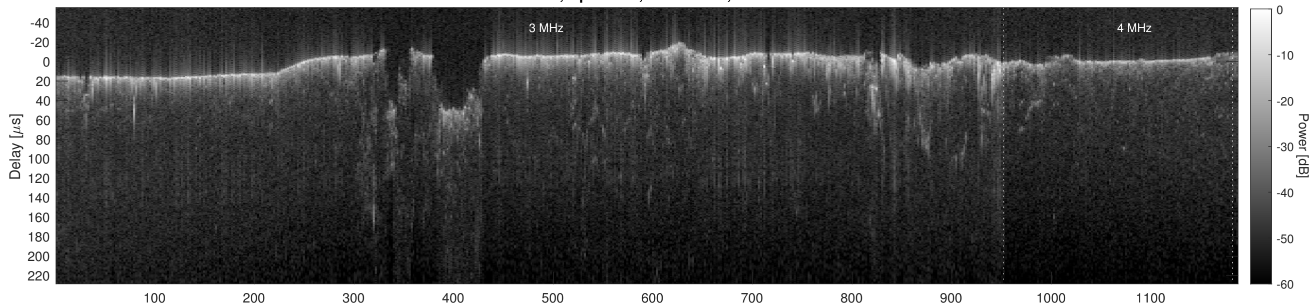
Orbit 4957, Cluttergram
