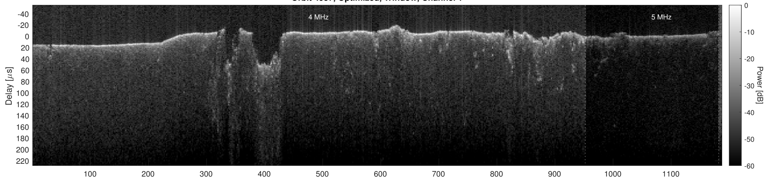
Orbit 4957, Optimized, Window, Channel 2
