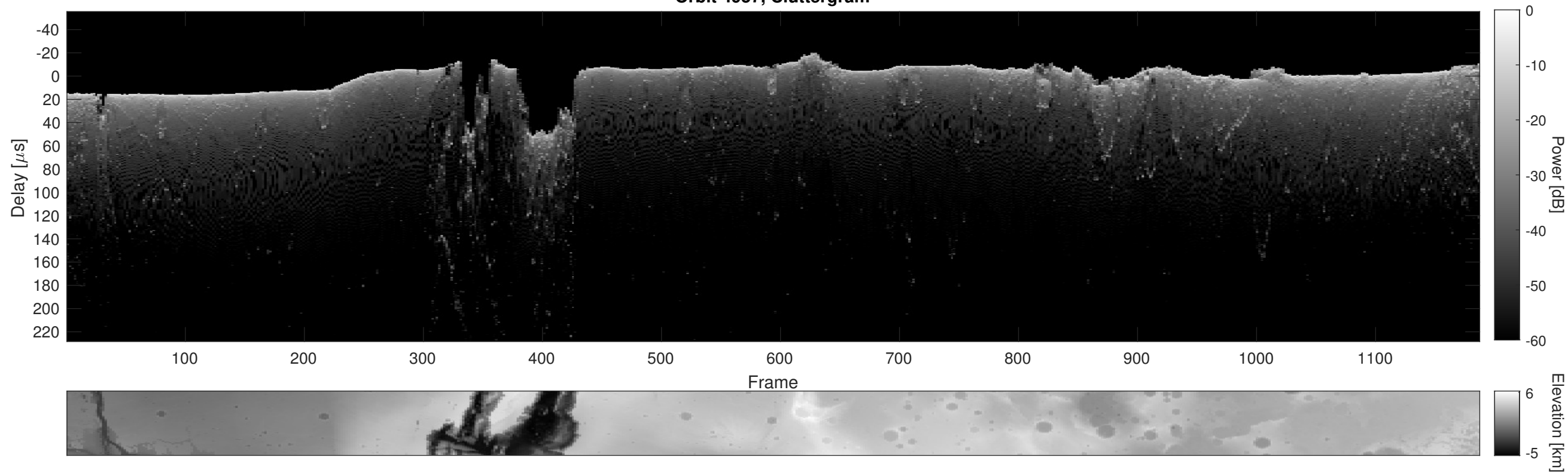
Orbit 4957, Cluttergram
