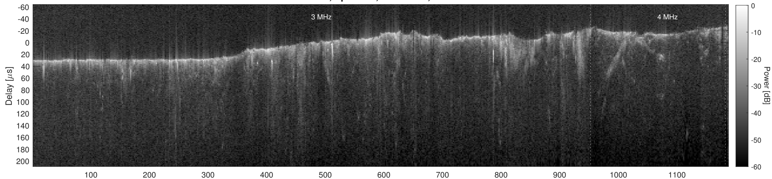
Orbit 4958, Cluttergram
