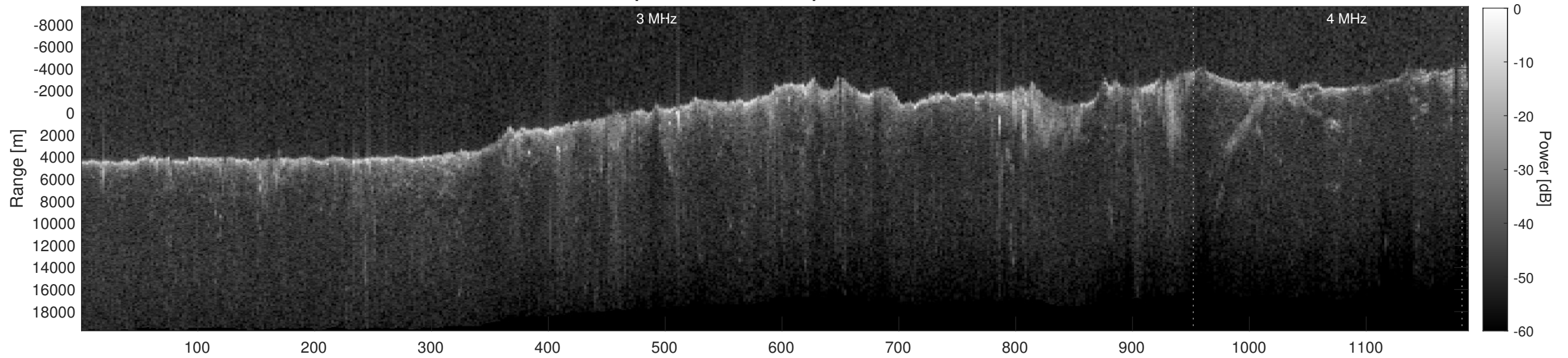
Orbit 4958, Depth-Corrected Cluttergram
