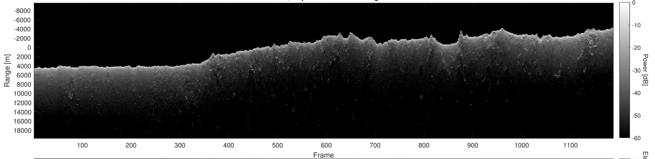
Orbit 4958, Depth-Corrected Cluttergram
