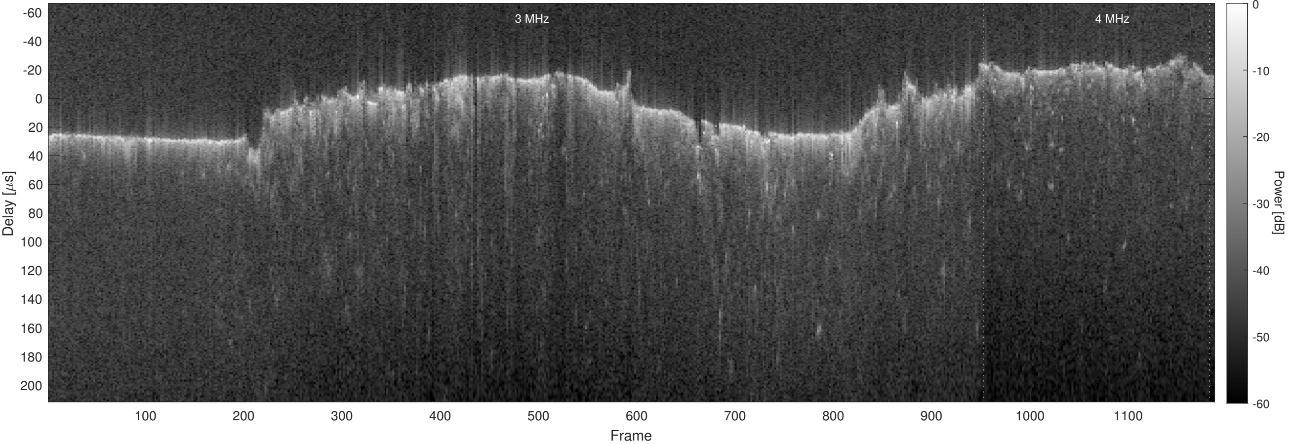
Orbit 4959, Optimized, No Window, Channel 2
