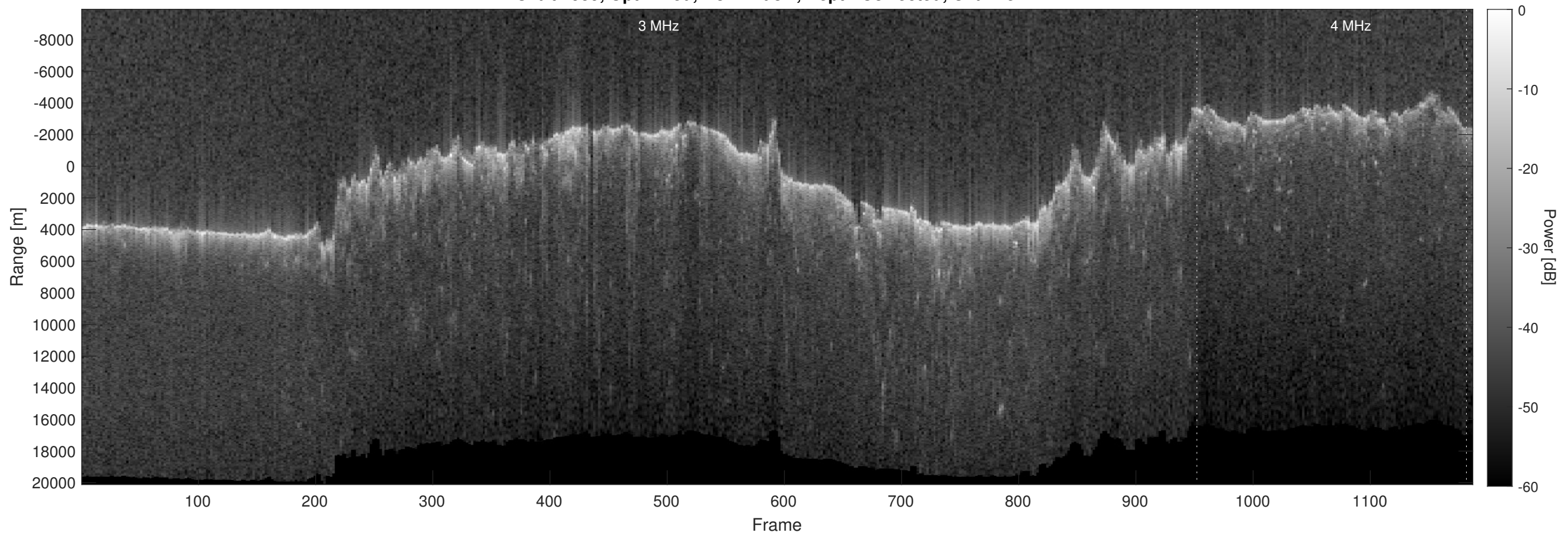
Orbit 4959, Optimized, No Window, Depth-Corrected, Channel 2
