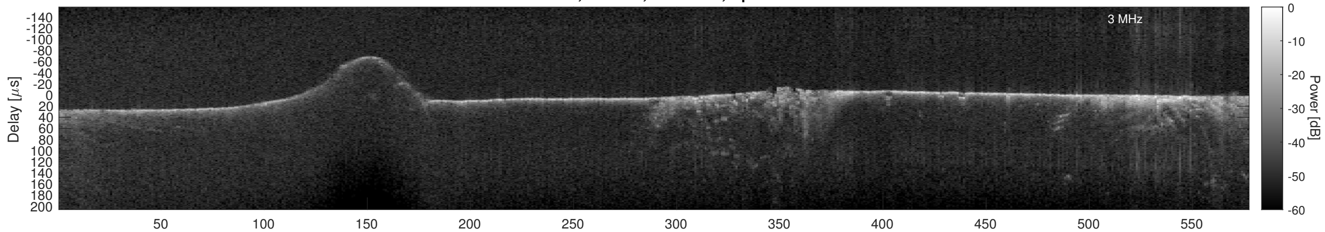
Orbit 4961, Cluttergram
