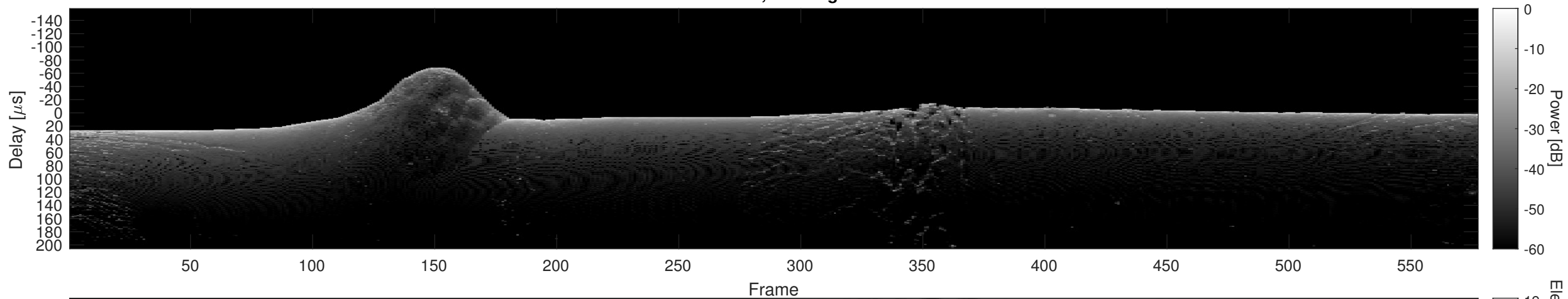
Orbit 4961, Cluttergram
