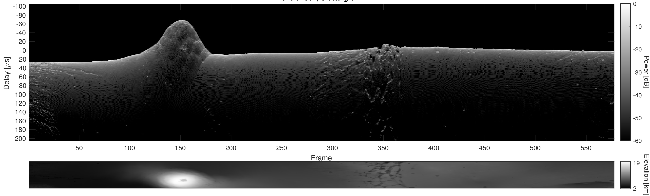
Orbit 4961, Cluttergram
