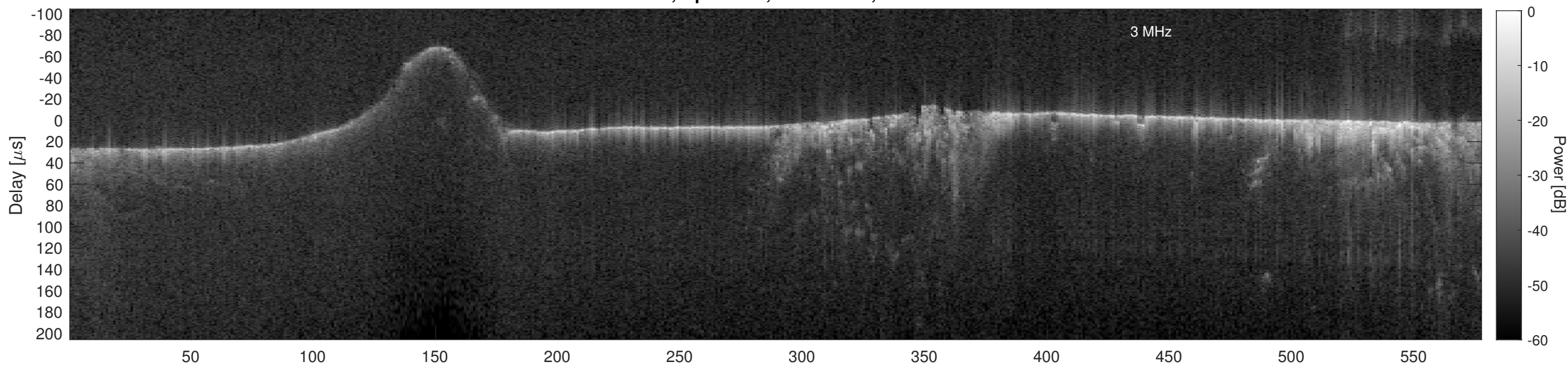
Orbit 4961, Cluttergram
