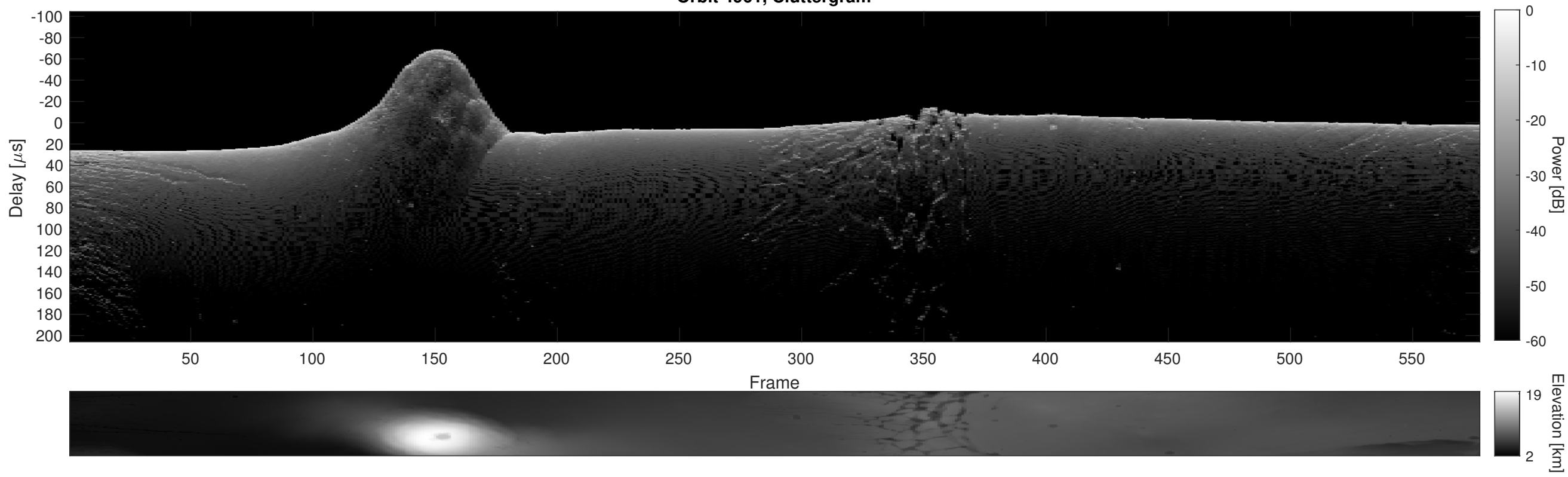
Orbit 4961, Cluttergram
