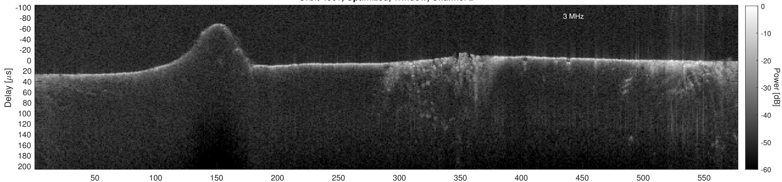
Orbit 4961, Cluttergram
