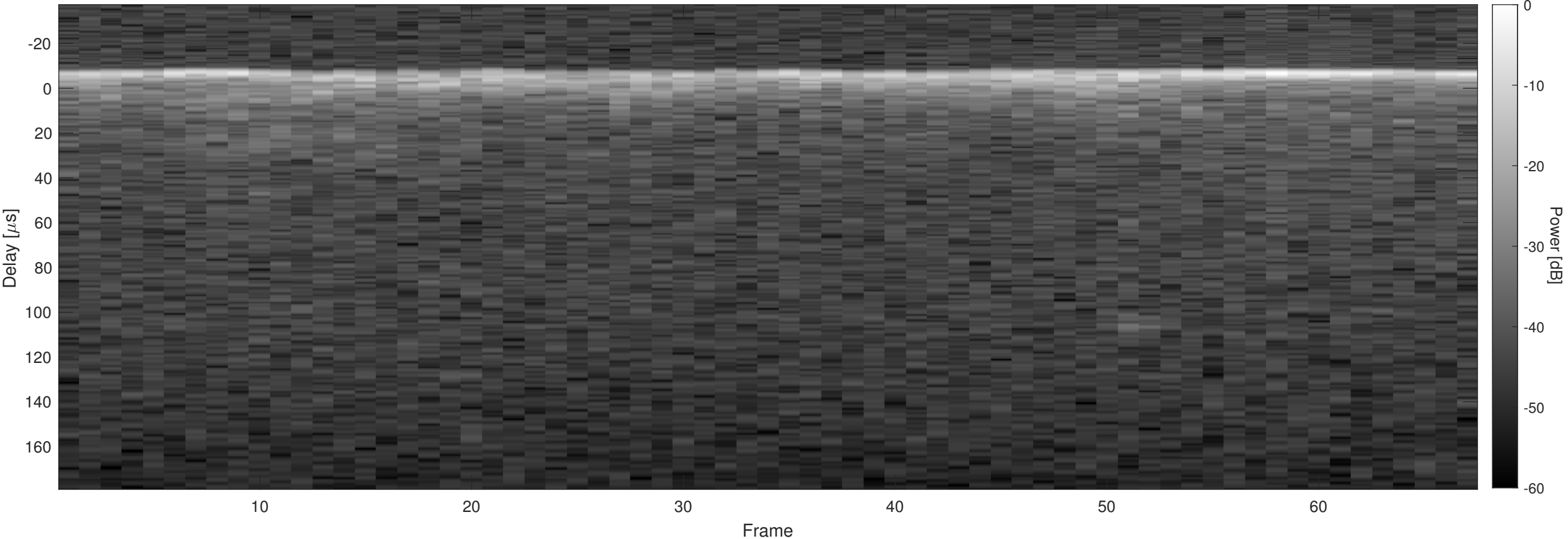
Orbit 4962, Chapman, Window, Channel 2
