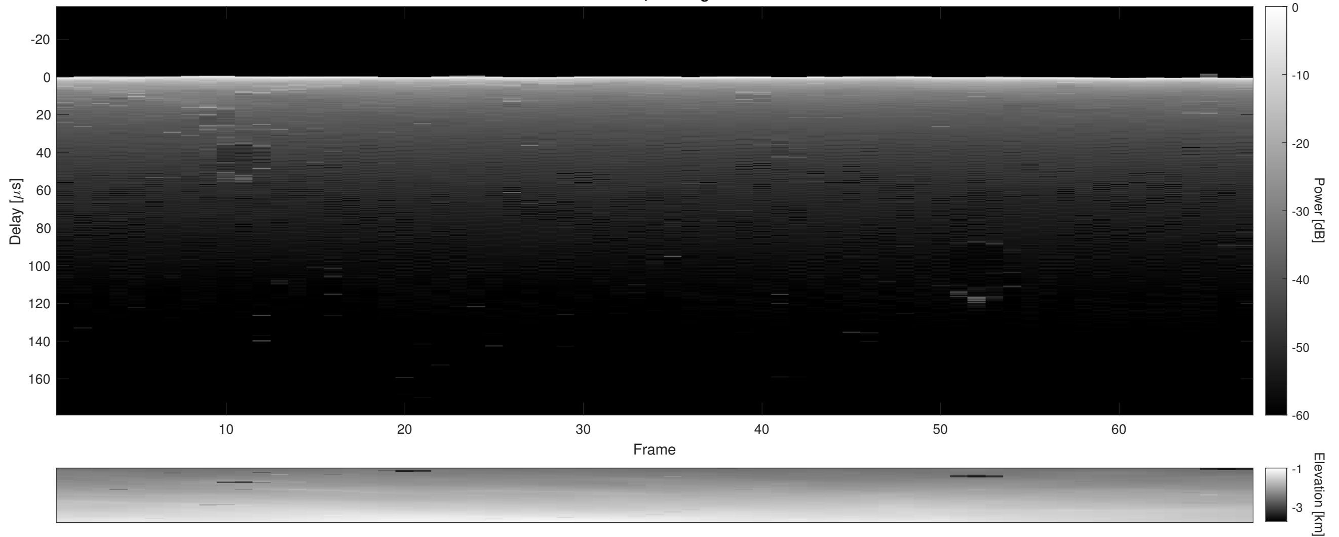
Orbit 4962, Cluttergram
