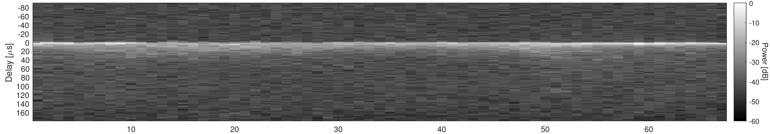
Orbit 4962, Cluttergram
