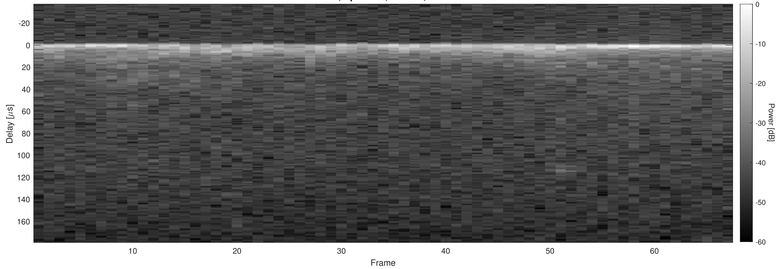
Orbit 4962, Optimized, Window, Channel 2
