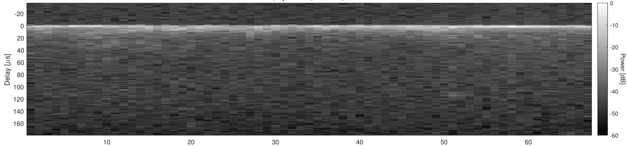
Orbit 4962, Optimized, Window, Channel 2
