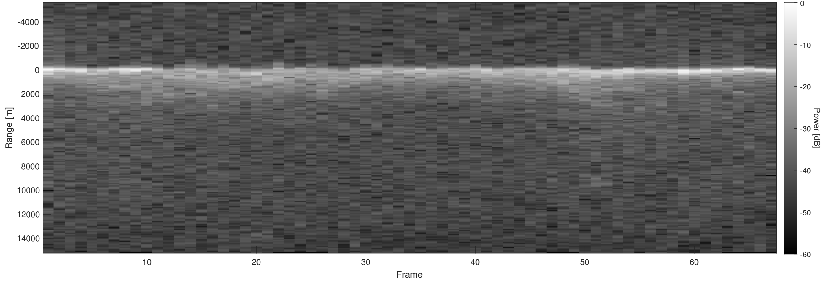
Orbit 4962, Optimized, Window, Depth-Corrected, Channel 2
