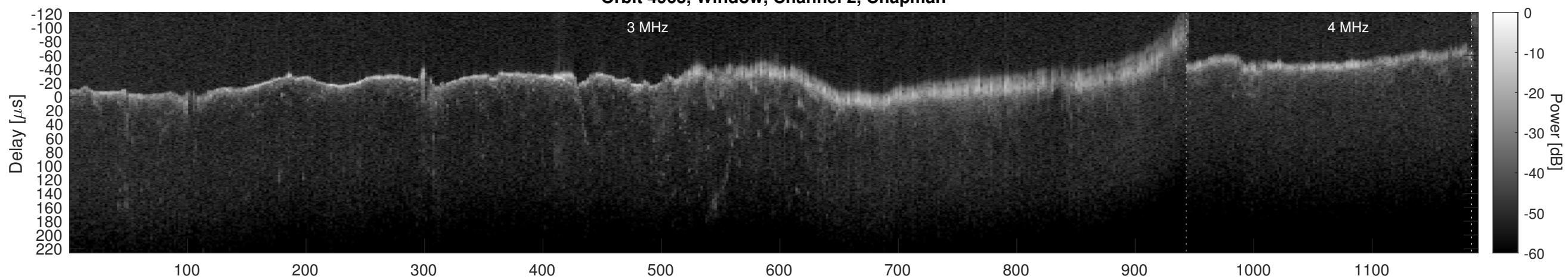
Orbit 4963, Window, Channel 2, Optimized
