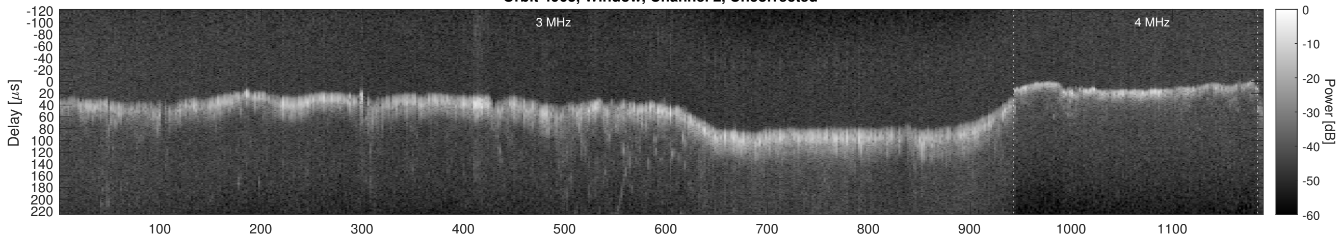
Orbit 4963, Window, Channel 2, Chapman
