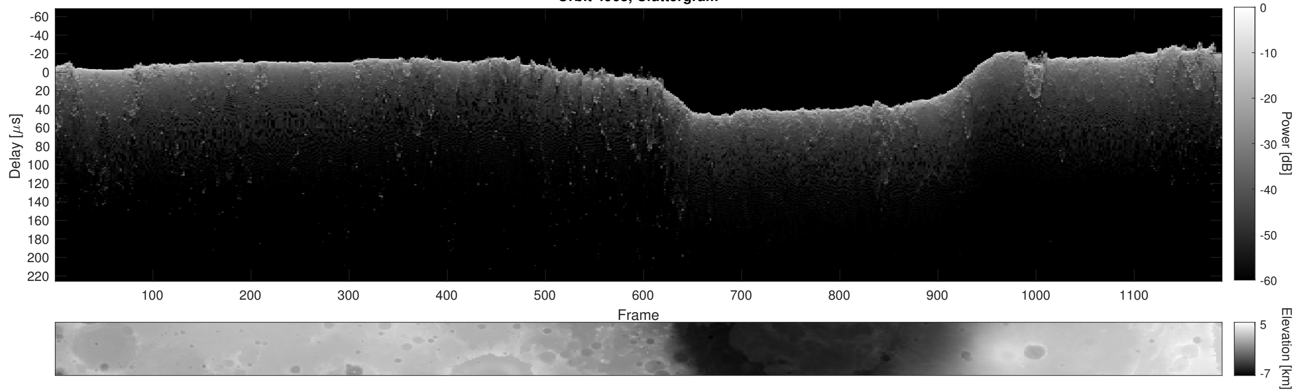
Orbit 4963, Cluttergram
