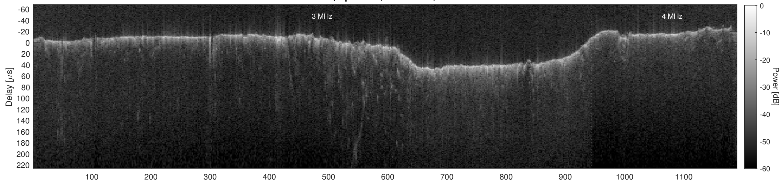
Orbit 4963, Cluttergram
