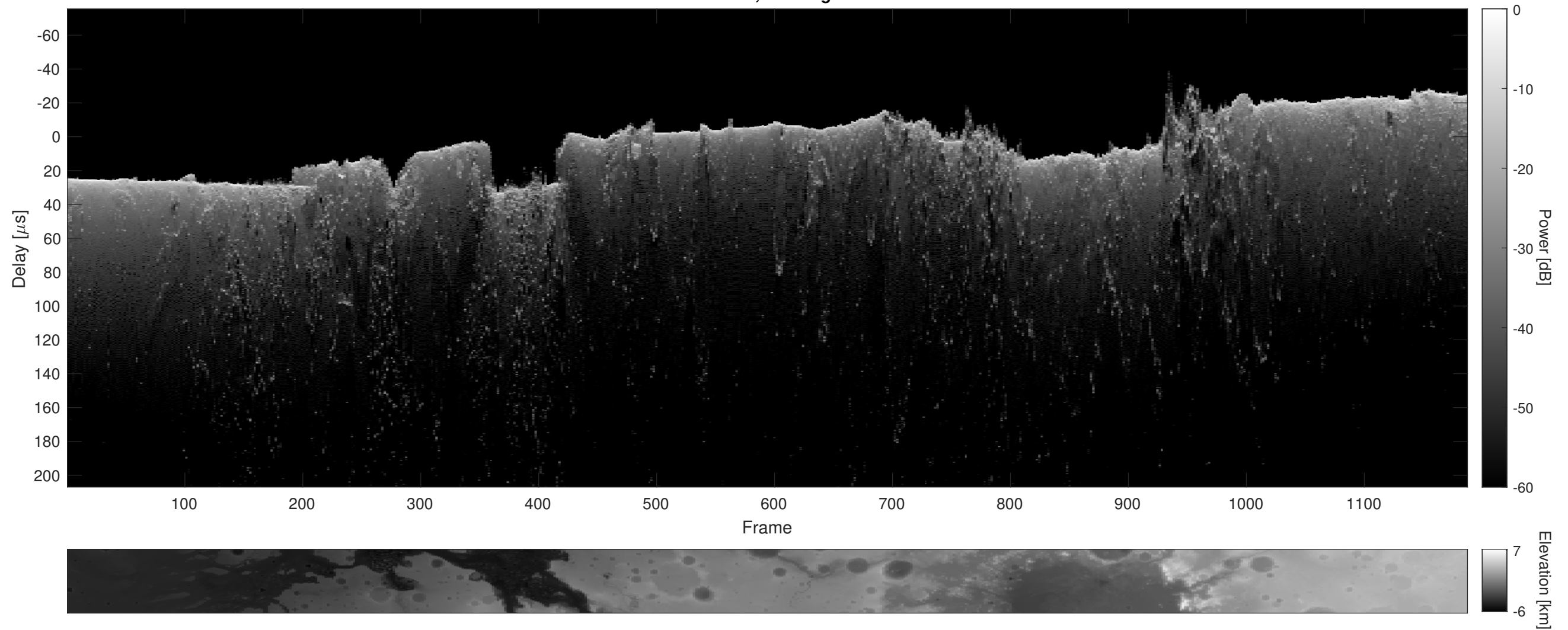
Orbit 4964, Cluttergram
