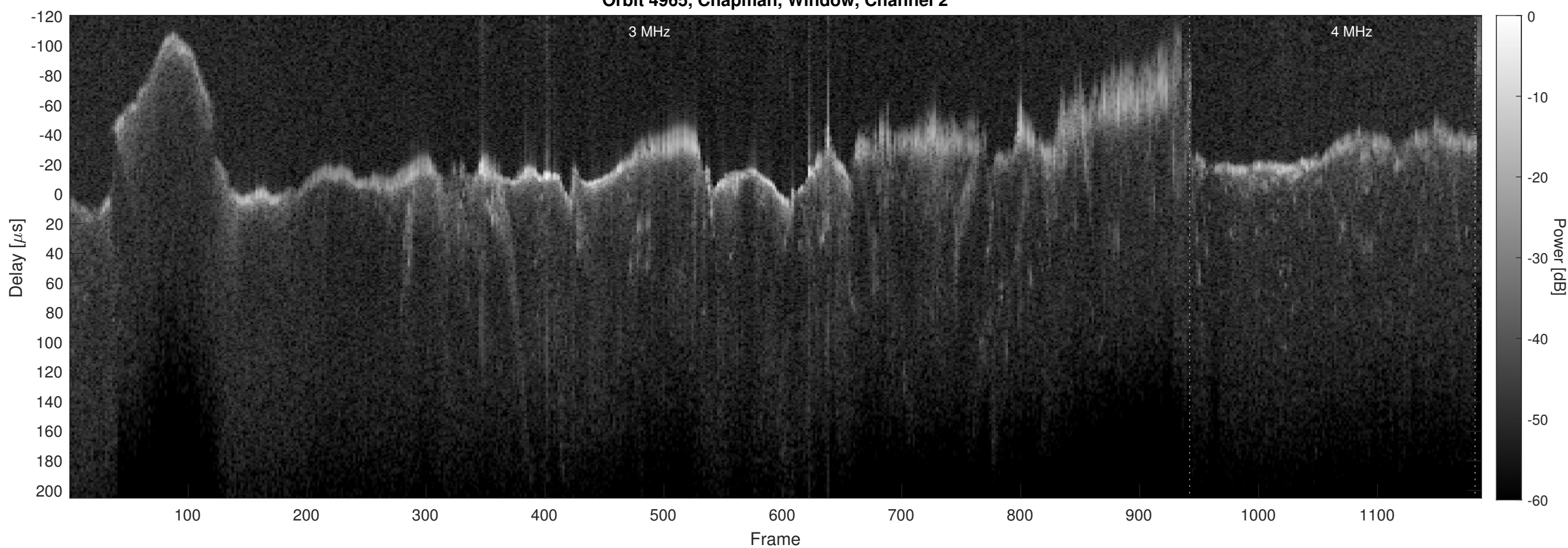
Orbit 4965, Chapman, Window, Channel 2
