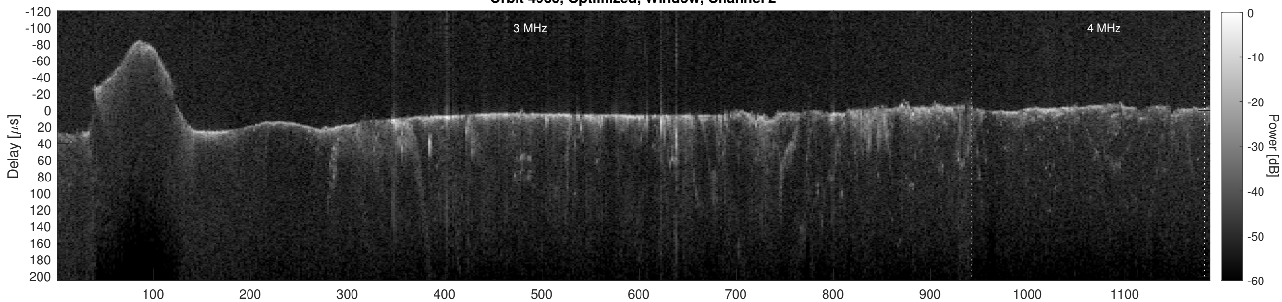
Orbit 4965, Cluttergram
