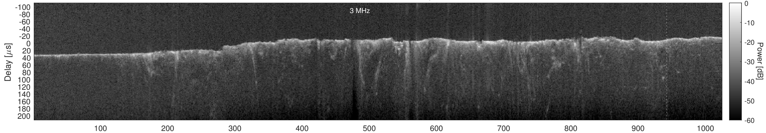
Orbit 4966, Cluttergram
