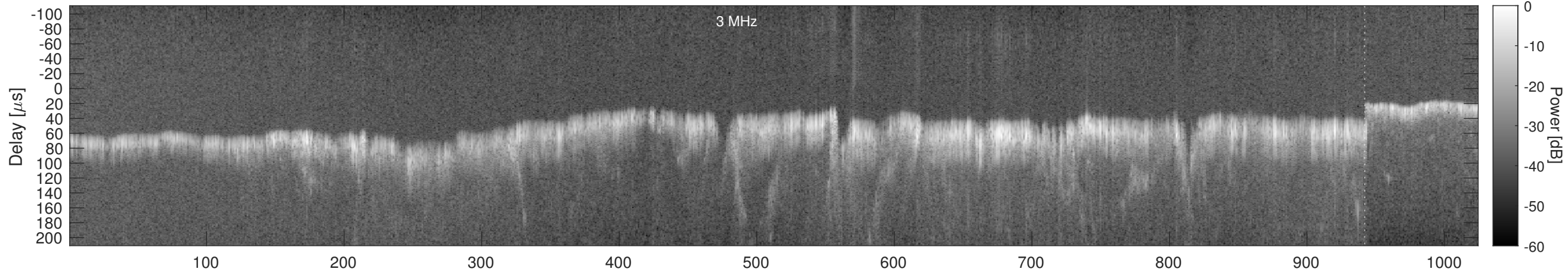
Orbit 4966, Window, Channel 2, Chapman
