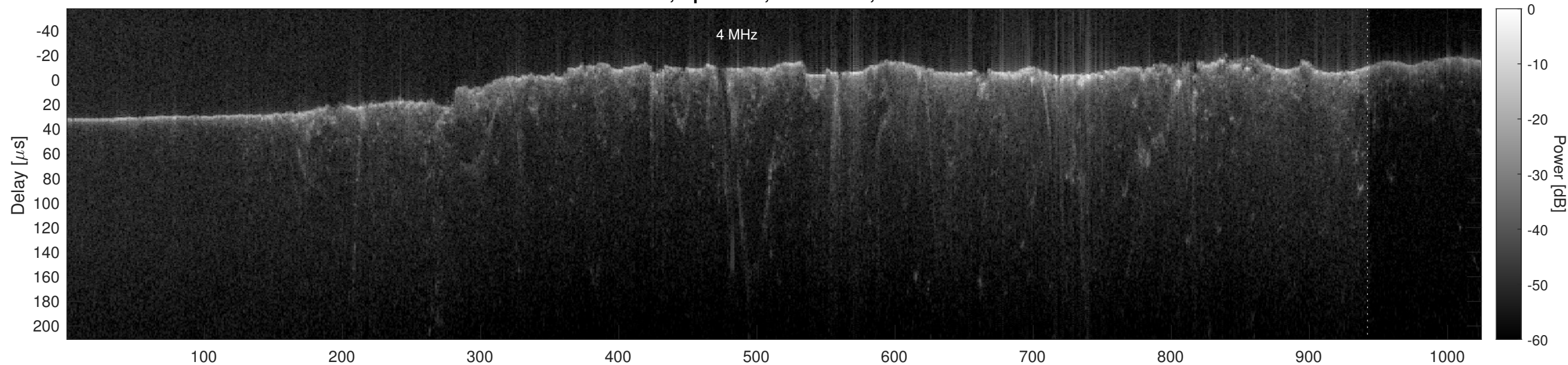
Orbit 4966, Optimized, No Window, Channel 2
