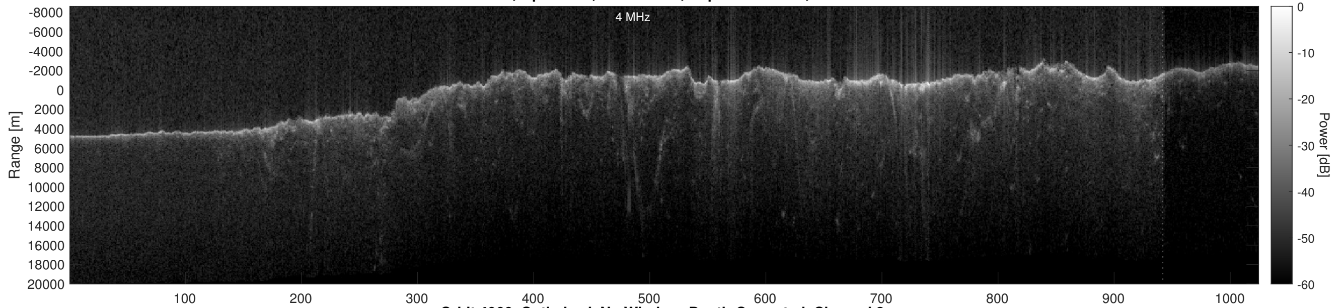
Orbit 4966, Optimized, No Window, Depth-Corrected, Channel 2
