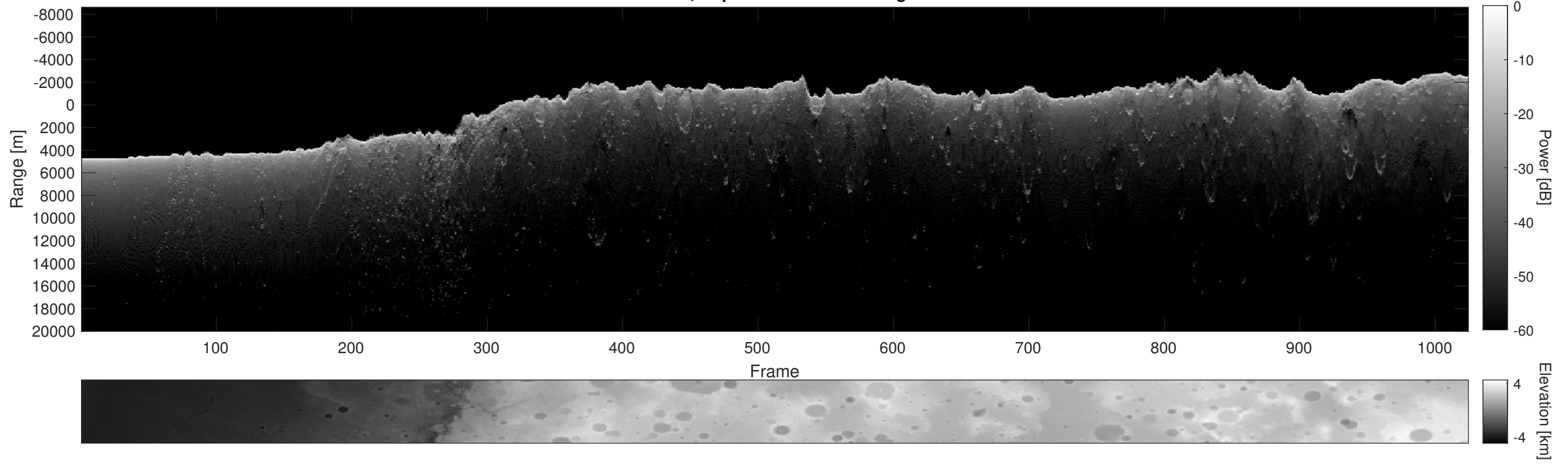
Orbit 4966, Depth-Corrected Cluttergram
