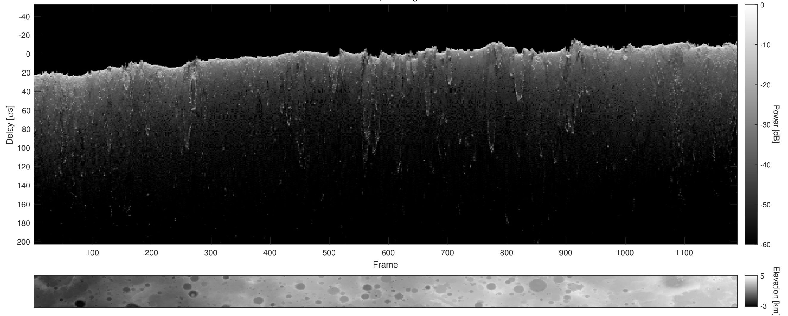
Orbit 4967, Cluttergram
