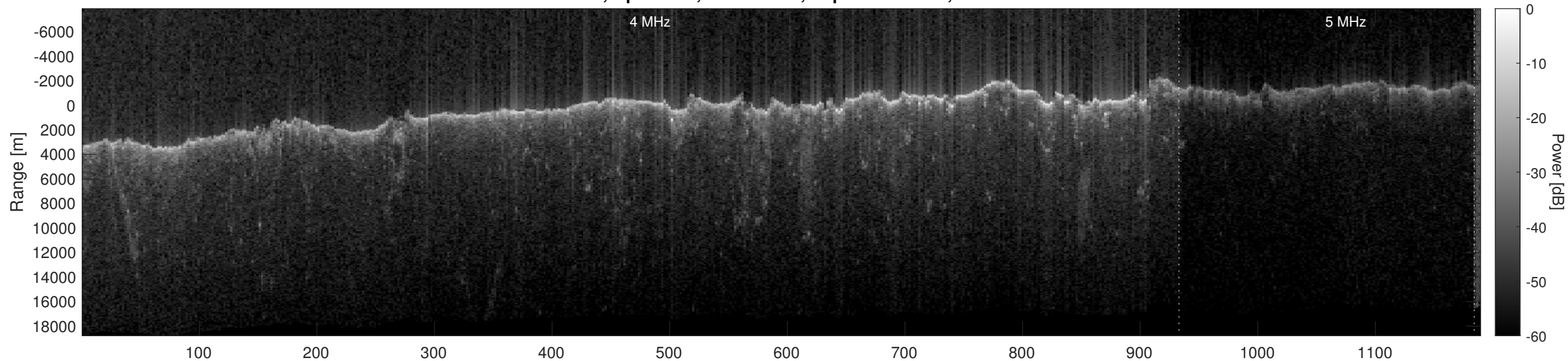
Orbit 4967, Optimized, No Window, Depth-Corrected, Channel 2
