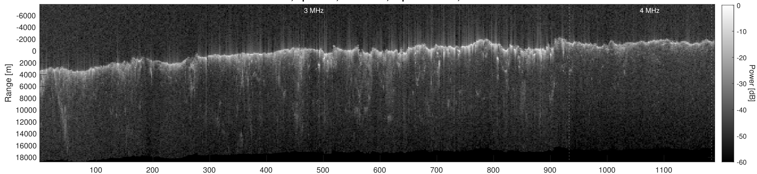
Orbit 4967, Depth-Corrected Cluttergram
