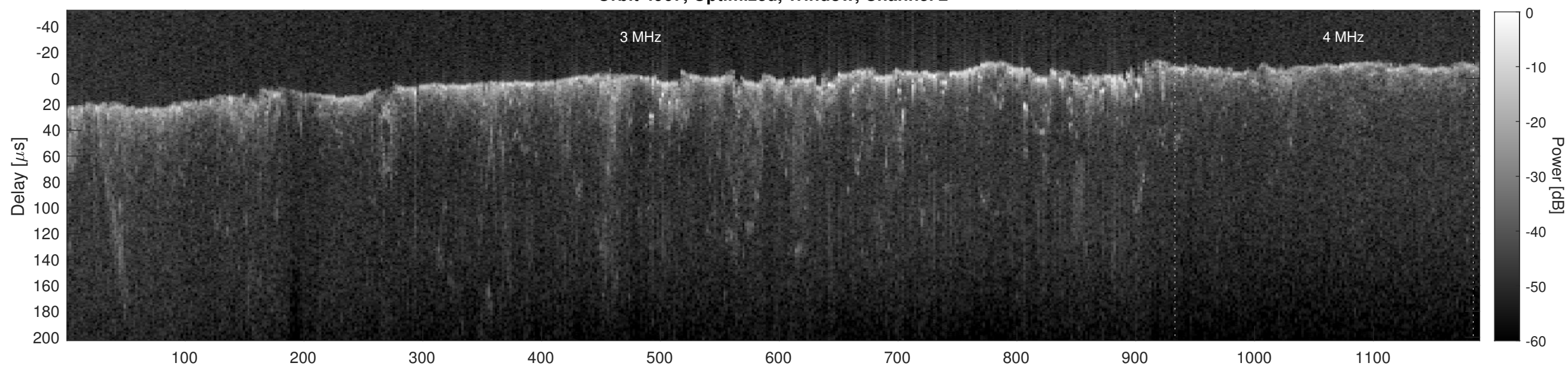
Orbit 4967, Cluttergram
