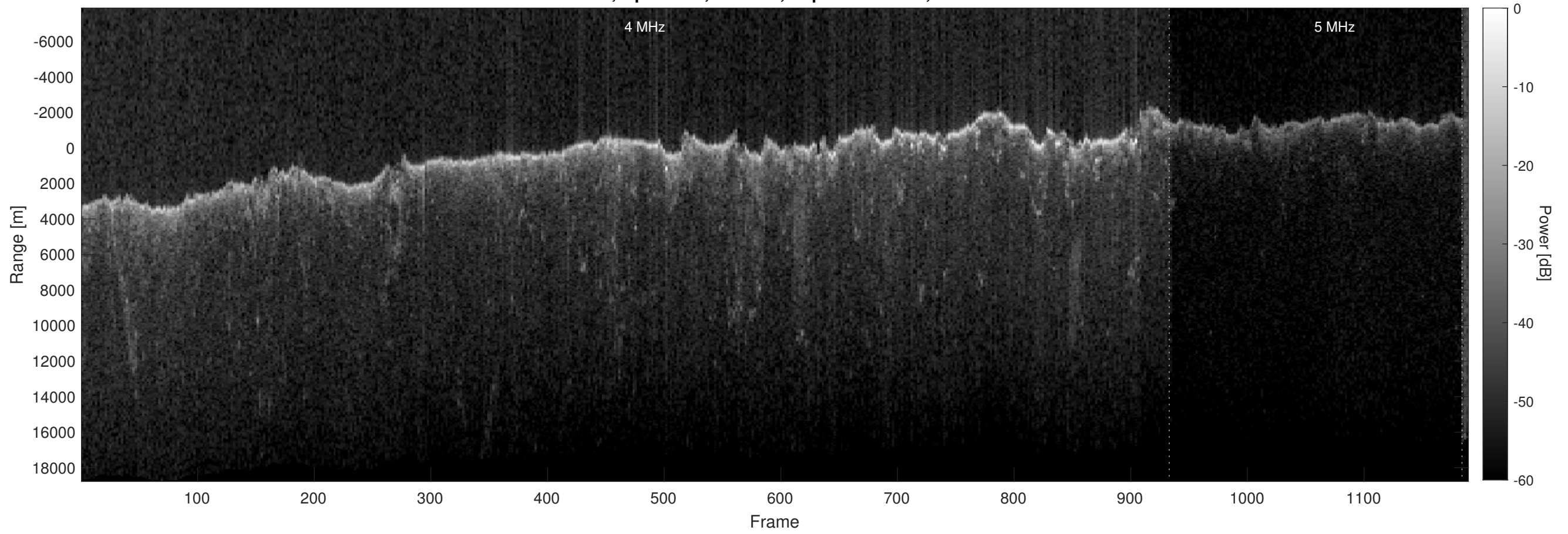
Orbit 4967, Optimized, Window, Depth-Corrected, Channel 2
