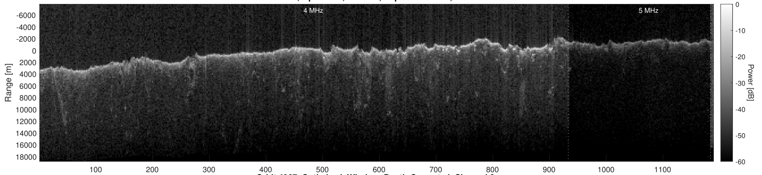
Orbit 4967, Optimized, Window, Depth-Corrected, Channel 2
