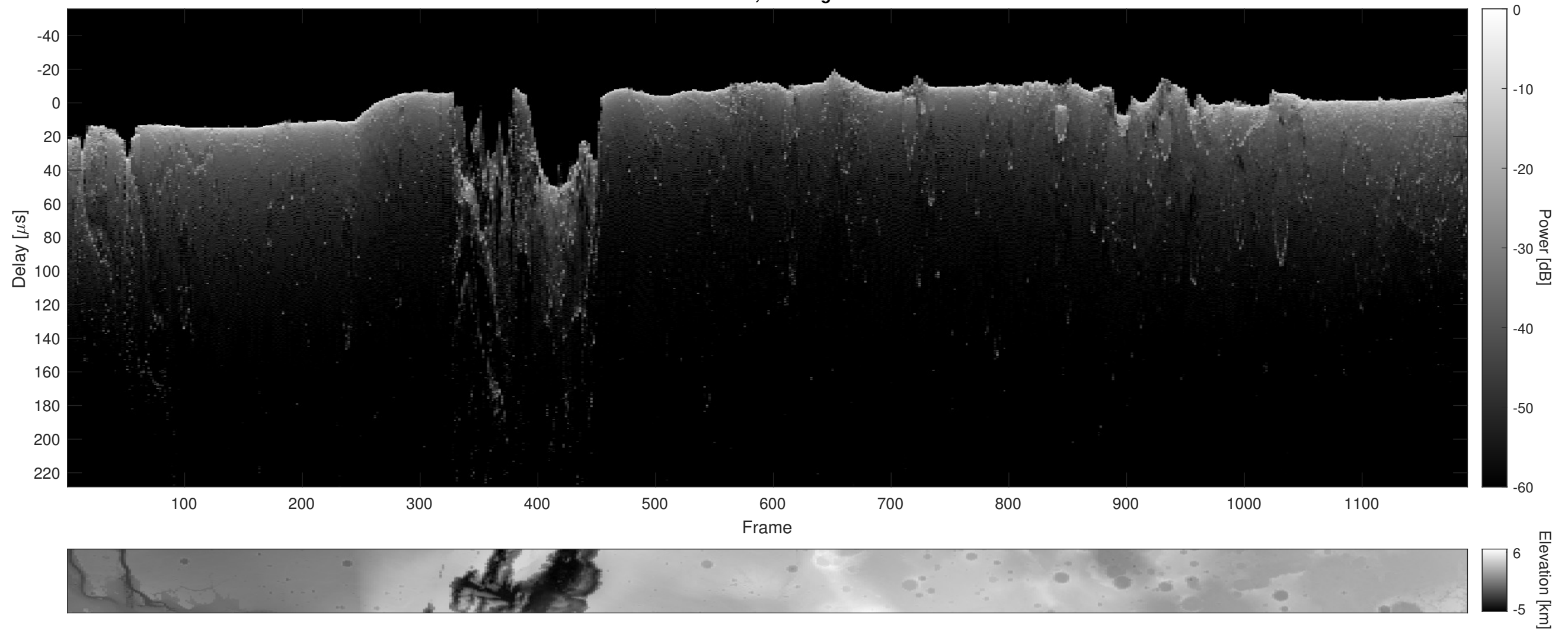
Orbit 4968, Cluttergram
