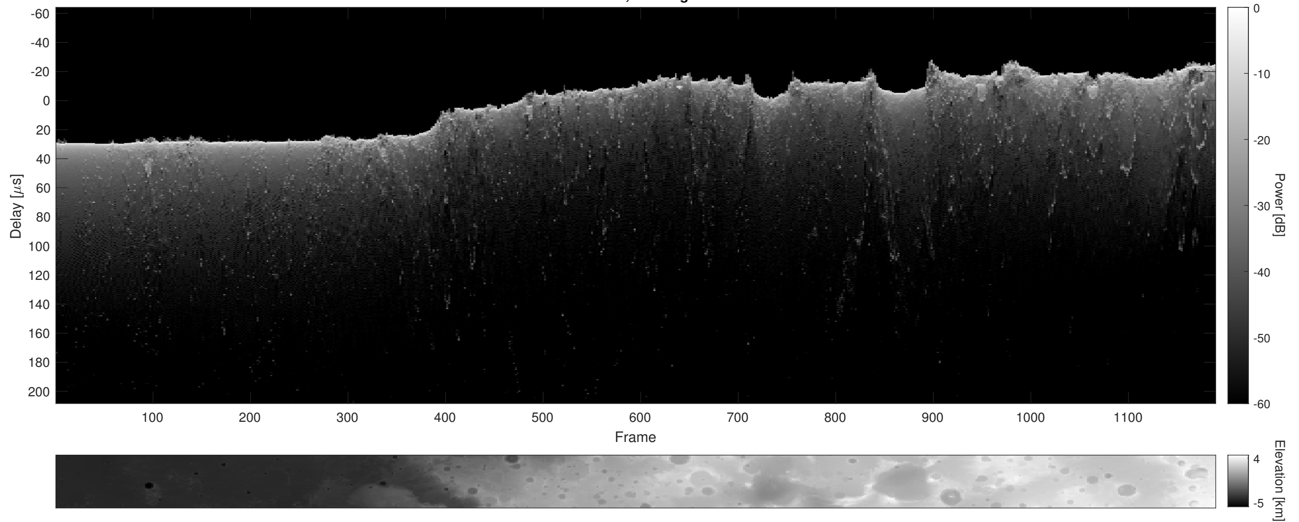
Orbit 4969, Cluttergram
