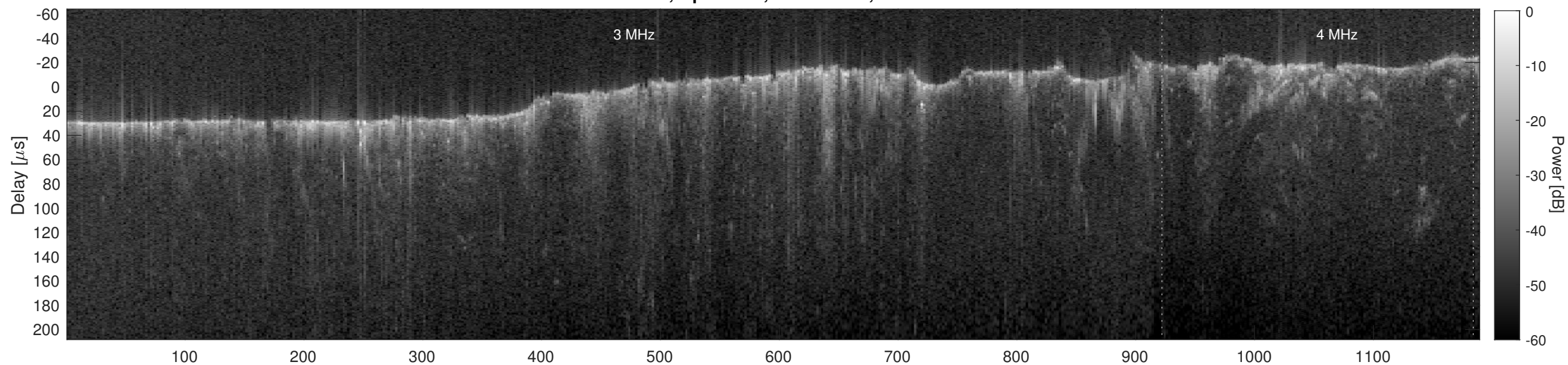
Orbit 4969, Cluttergram
