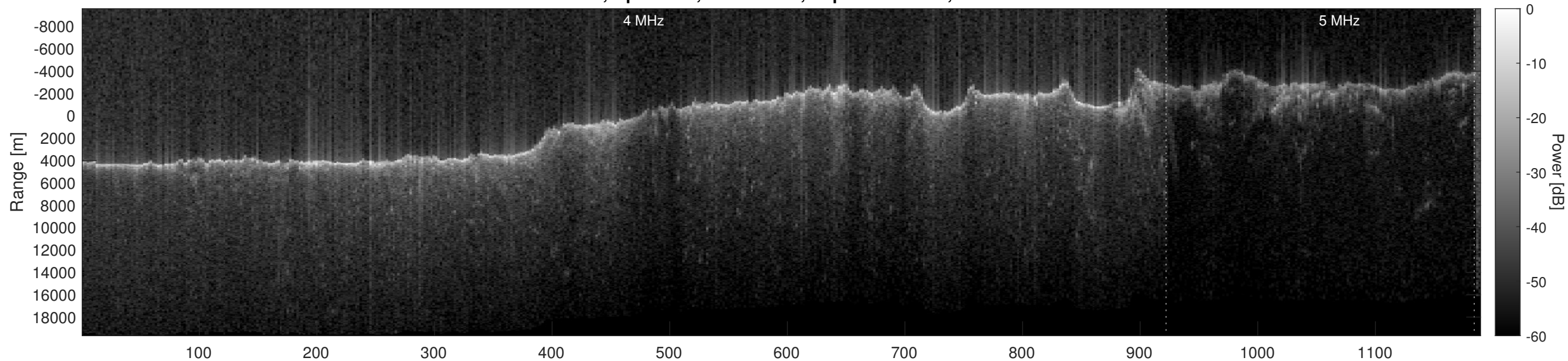
Orbit 4969, Optimized, No Window, Depth-Corrected, Channel 2
