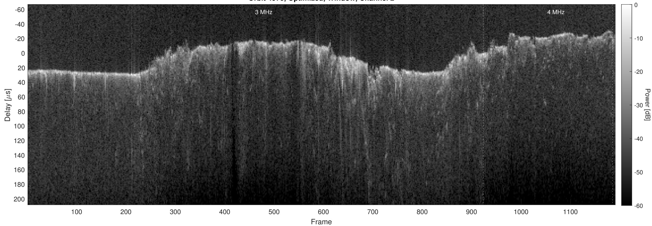
Orbit 4970, Optimized, Window, Channel 2
