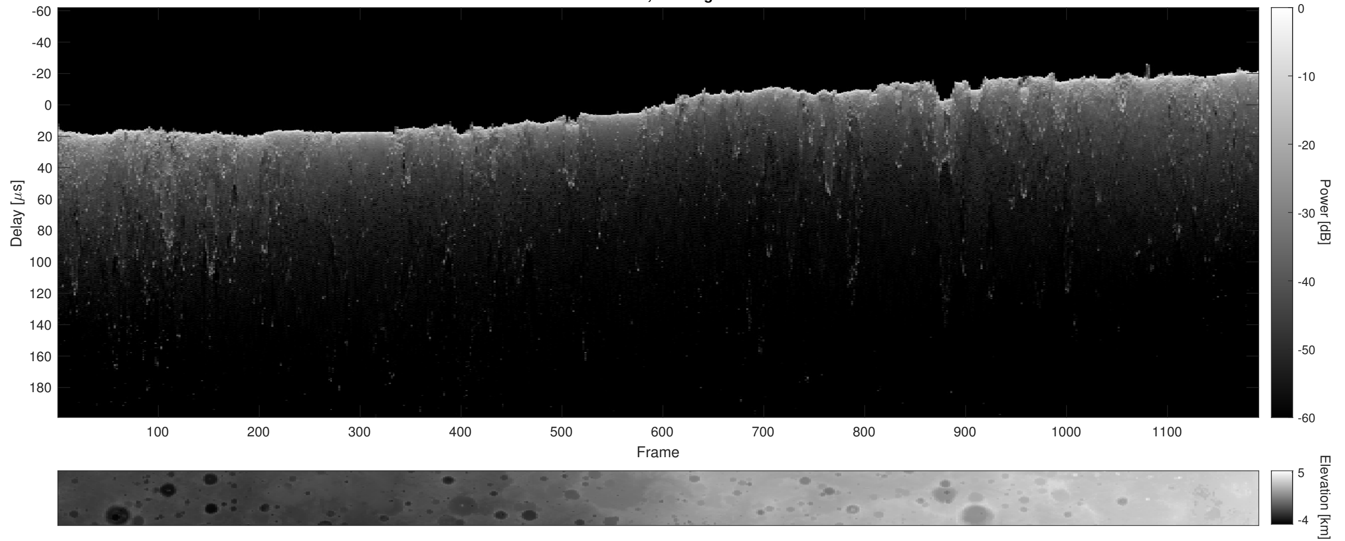
Orbit 4971, Cluttergram
