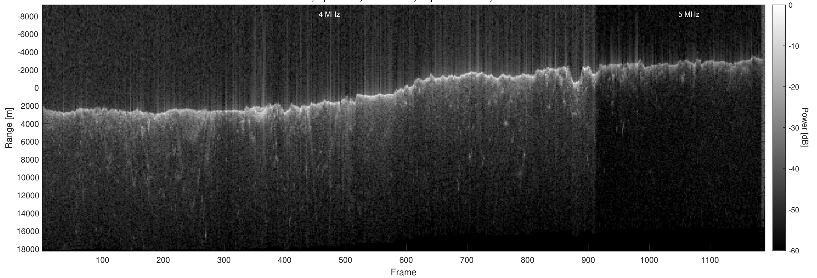
Orbit 4971, Optimized, No Window, Depth-Corrected, Channel 2
