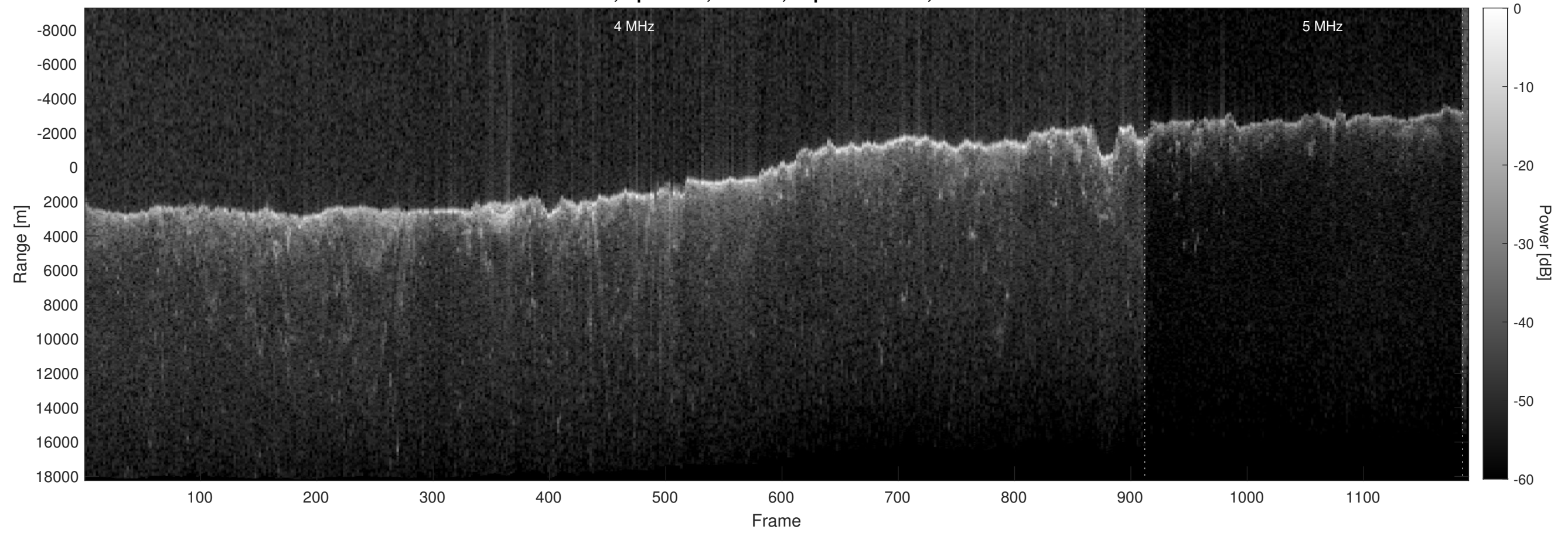
Orbit 4971, Optimized, Window, Depth-Corrected, Channel 2
