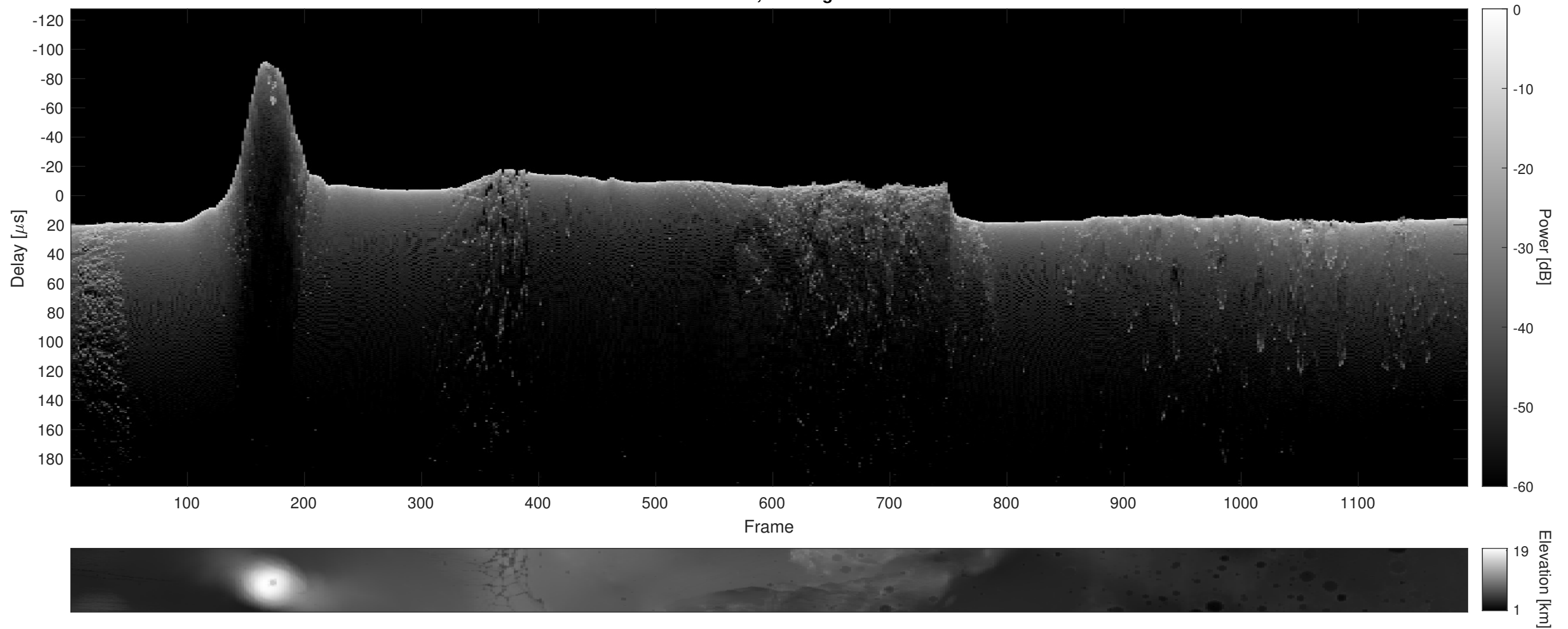
Orbit 4972, Cluttergram
