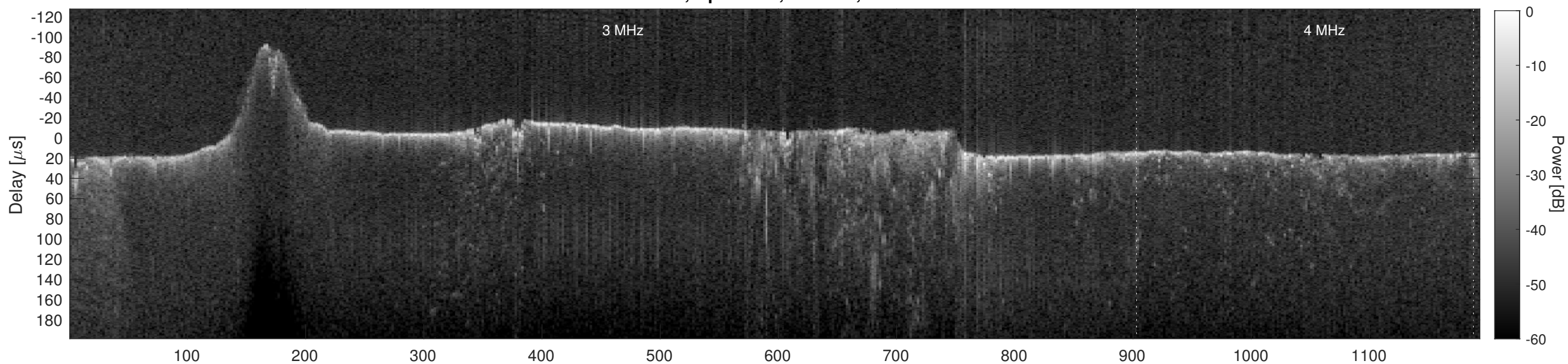
Orbit 4972, Cluttergram
