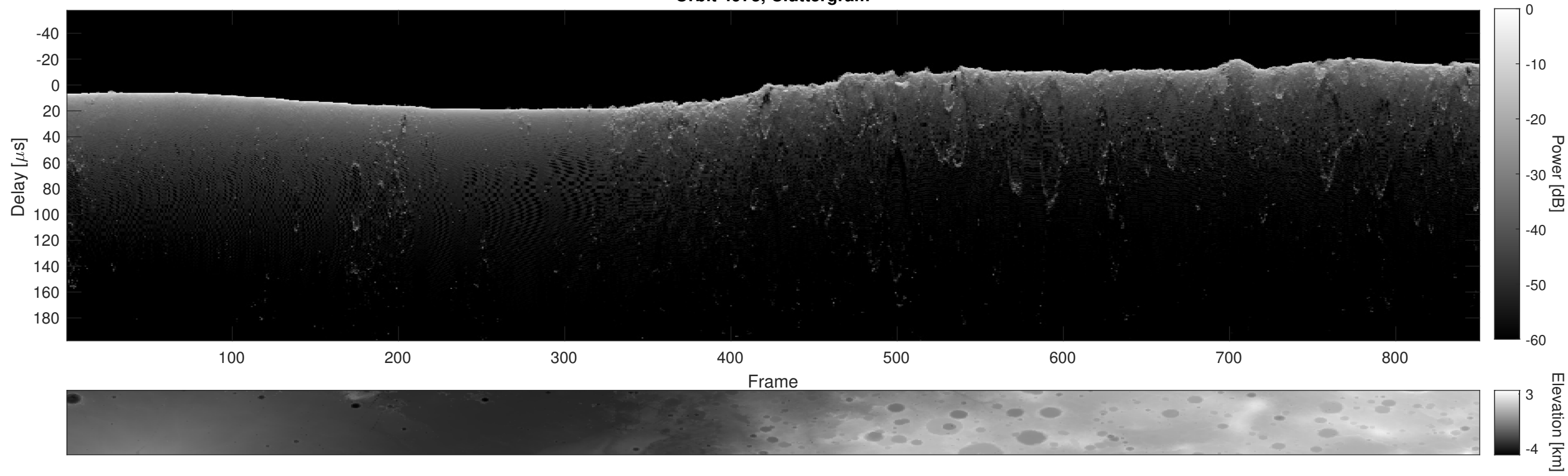
Orbit 4973, Cluttergram
