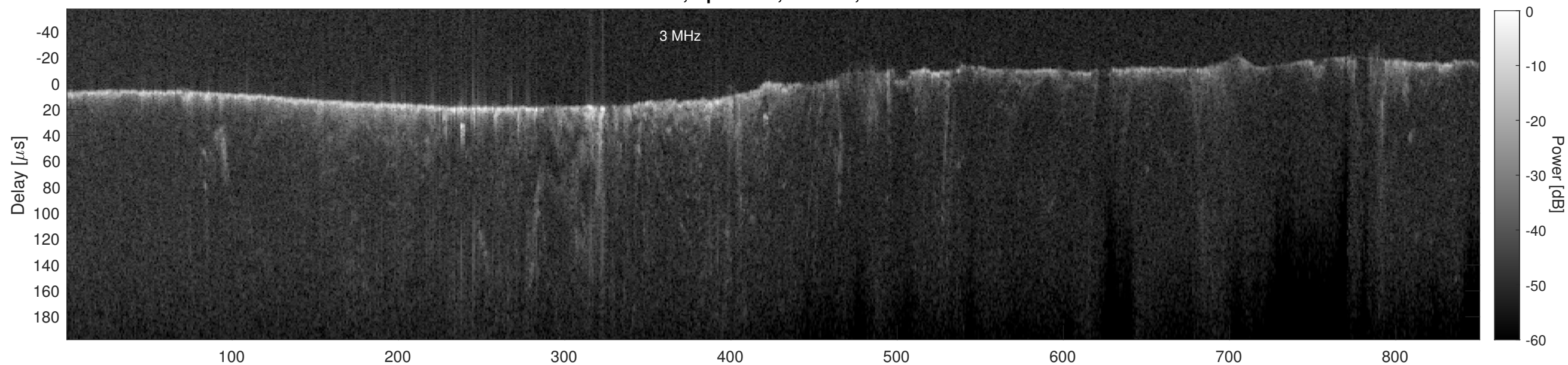
Orbit 4973, Cluttergram
