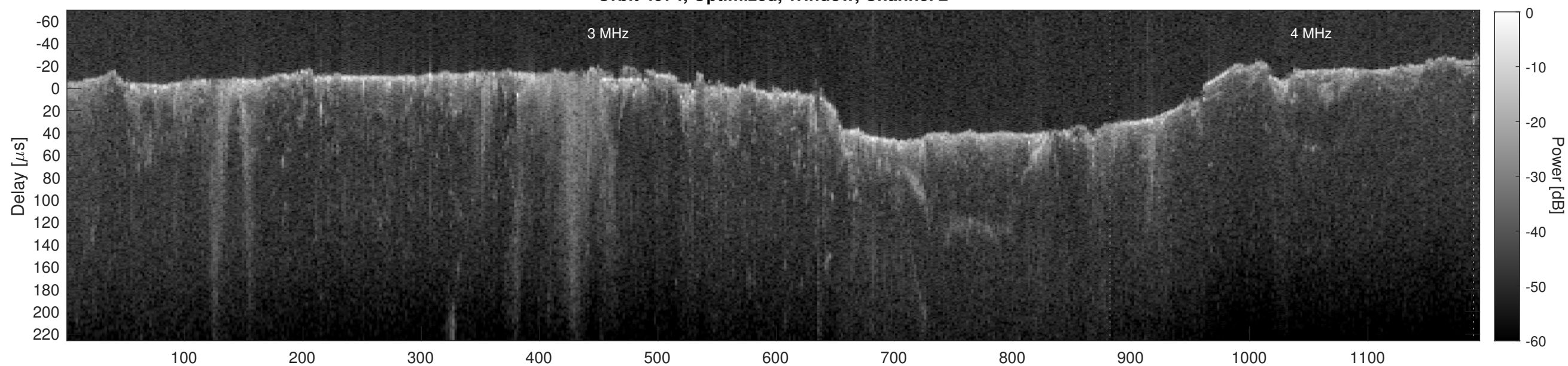
Orbit 4974, Cluttergram
