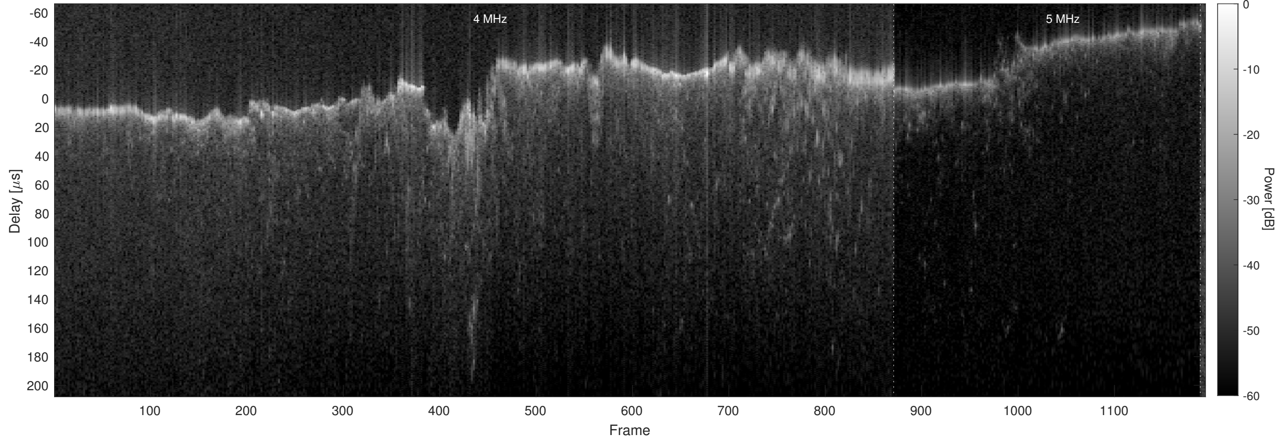
Orbit 4975, Chapman, No Window, Channel 2
